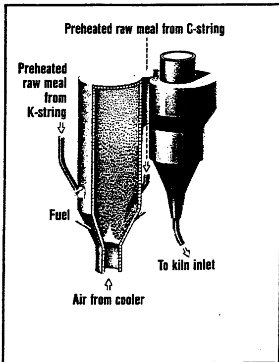
SLC calciner.
